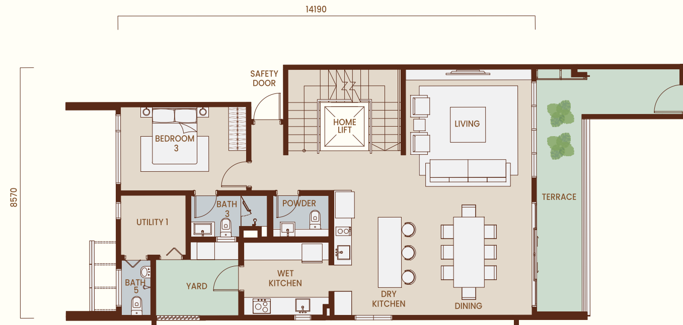
2nd Floor 1,198 sq. ft.
